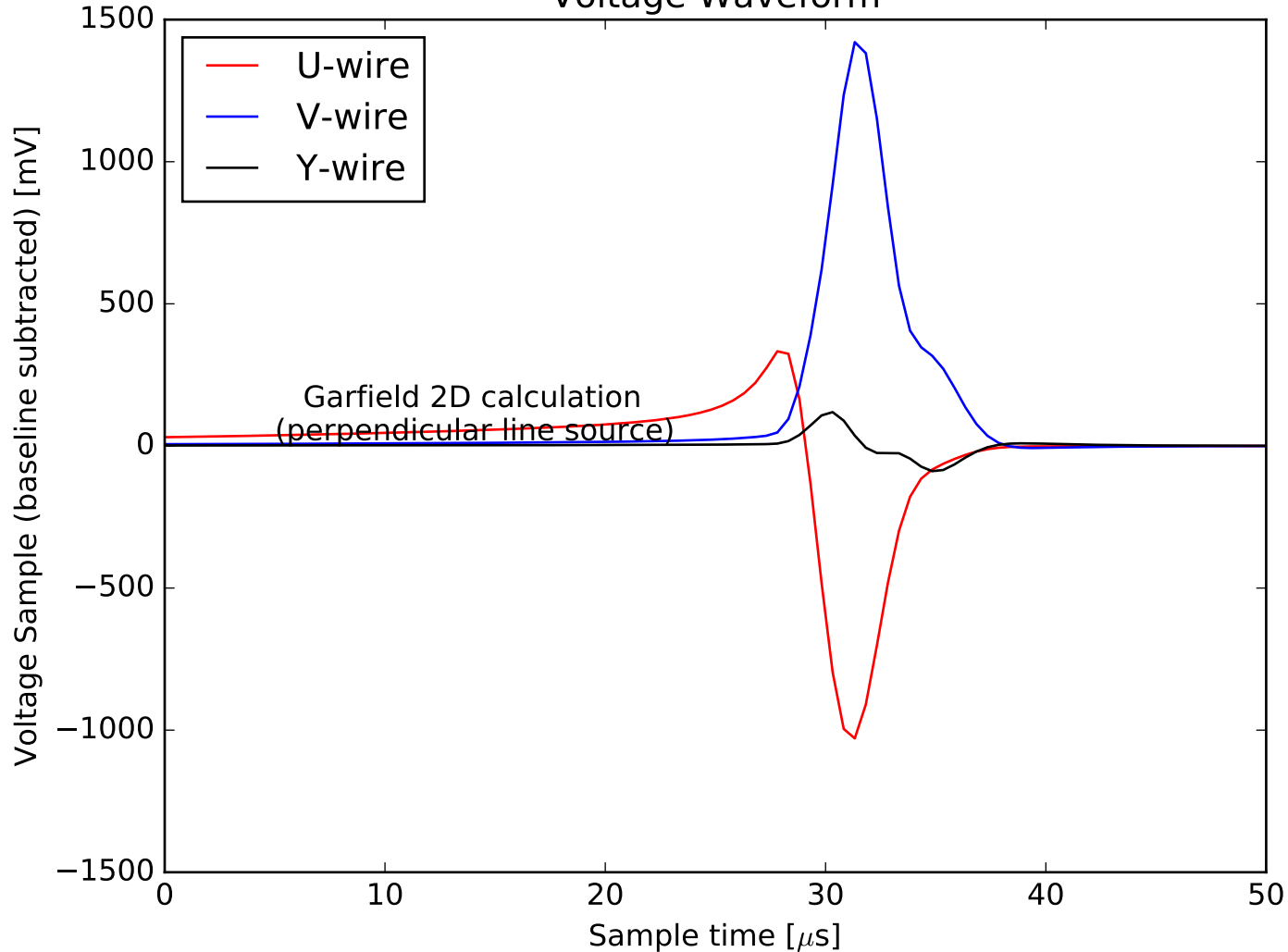
Voltage Waveform
