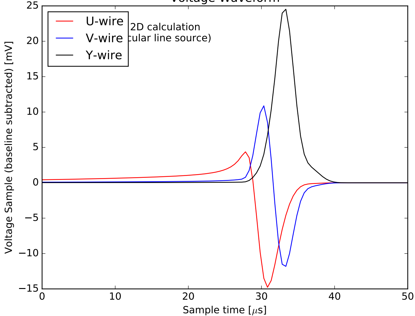
Voltage Waveform
