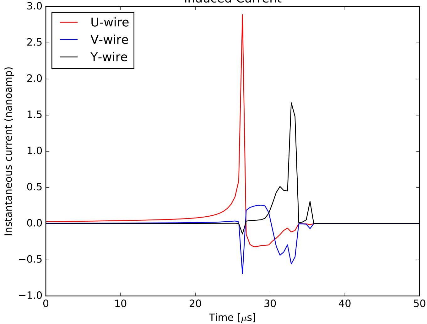
Induced Current
