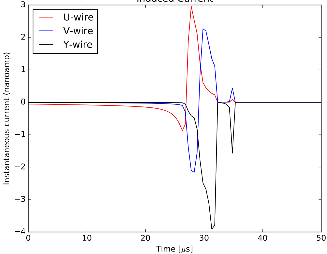
Induced Current
