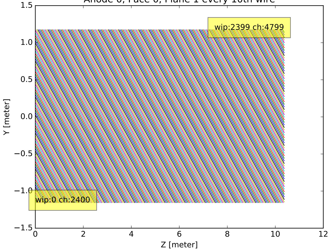
Anode 0, Face 0, Plane 1 every 10th wire
